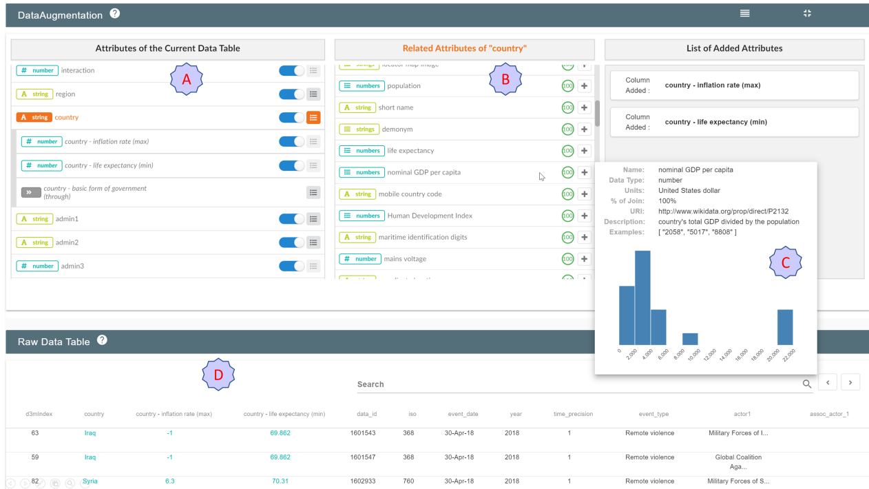
Fig. 2. The user interface of CAVA, showing an analysis session on the ACLED dataset. A shows the initial list of attributes in the table as well as augmented attributes, like the maximum inflation rate recorded for each country. The list of attributes related to the Country column is shown in B . Each related attribute is adorned with a donut chart showing the estimated join quality. Additional details about any attribute is available on demand in a popup, as seen in C . As attributes are added to the dataset during the analysis session, a preview of the table is updated as seen in D .
